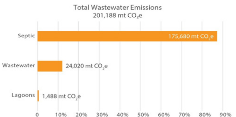
Figure 36. Total emissions and sources for waste and wastewater (mt CO 2 e).
