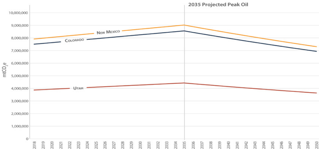
Figure 12. Projected oil and gas systems emissions from 2018-2050 (mt CO 2 e). 9
