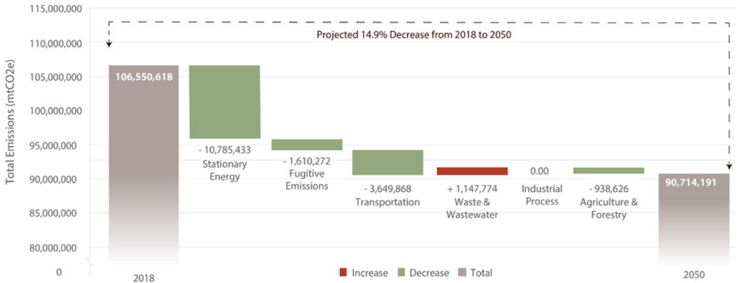
Figure 10. Colorado Plateau forecasted emissions change by sector from 2018-2050 (mt CO 2 e).
