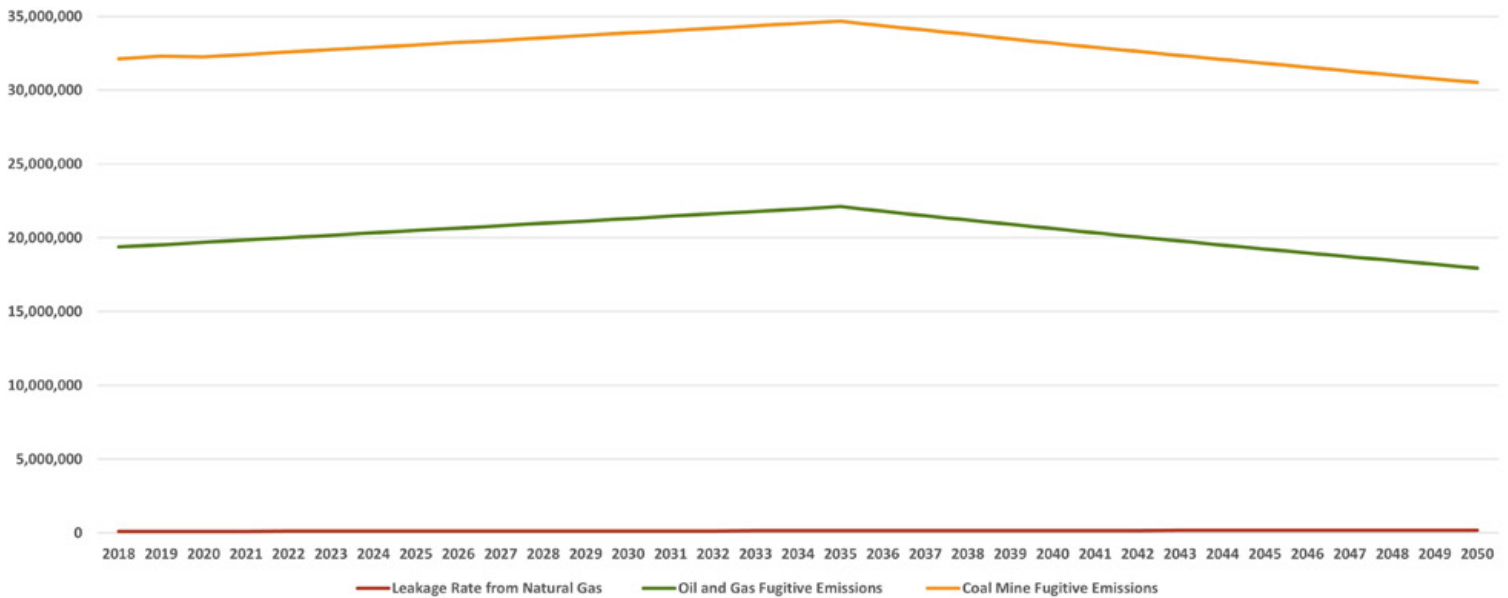
Figure 30. Forecasted emissions for fugitive emissions sector, 2018-2050 (mt CO 2 e).
