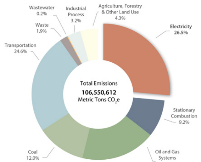
Figure 15. Proportion of total emissions from electricity.
