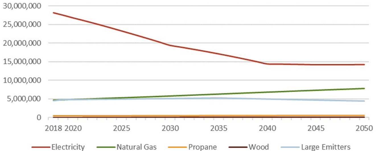
Figure 22. Forecasted emissions for electricity and stationary combustion, 2018-2050 (mt CO 2 e).
