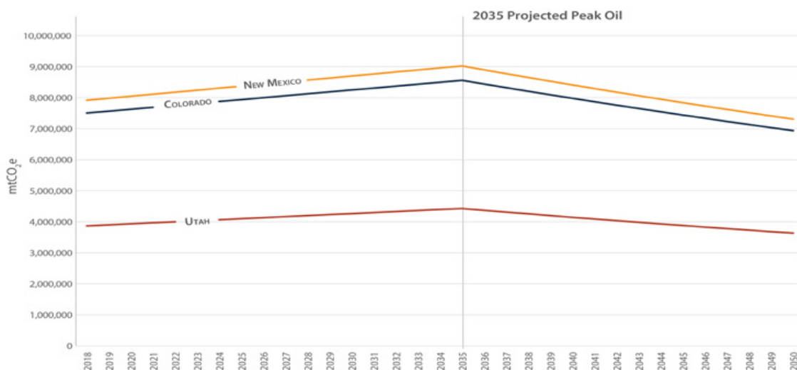
Figure 31. Projected oil and gas systems from 2018-2050 (mt CO 2 e).
