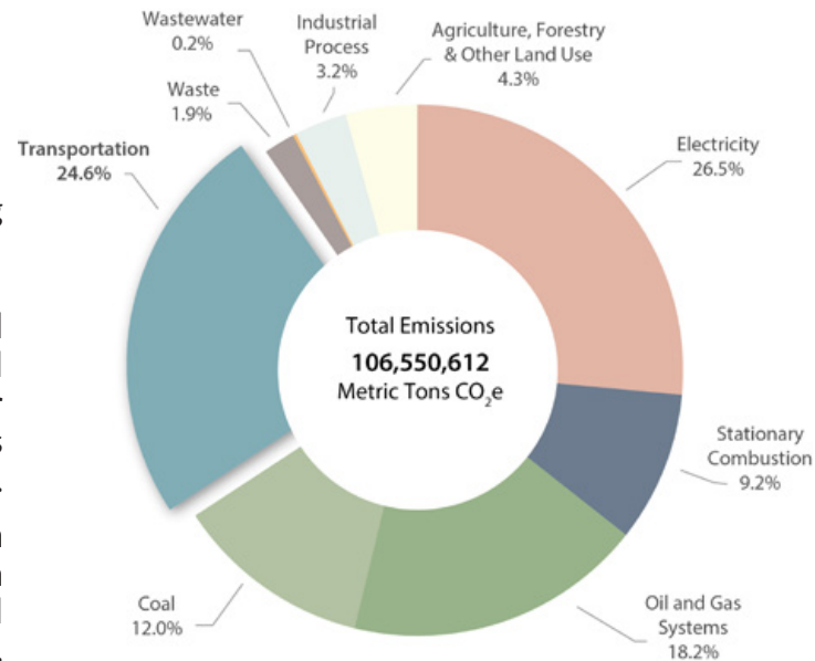
Figure 32. Proportion of total emissions from transportation.
