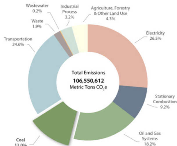
Figure 27. Proportion of total emissions from coal mining.
