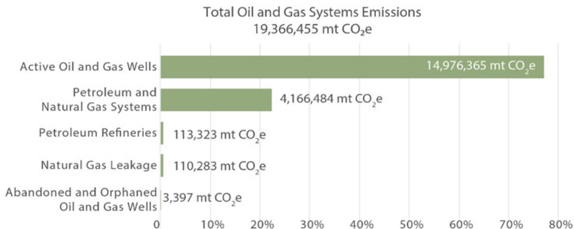
Figure 25. Total emissions sources for oil and gas systems (mt CO 2 e).
